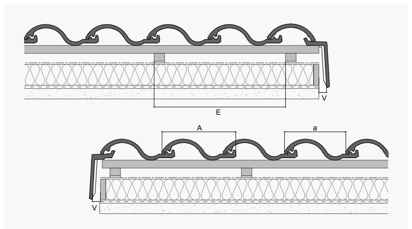
RIVES
